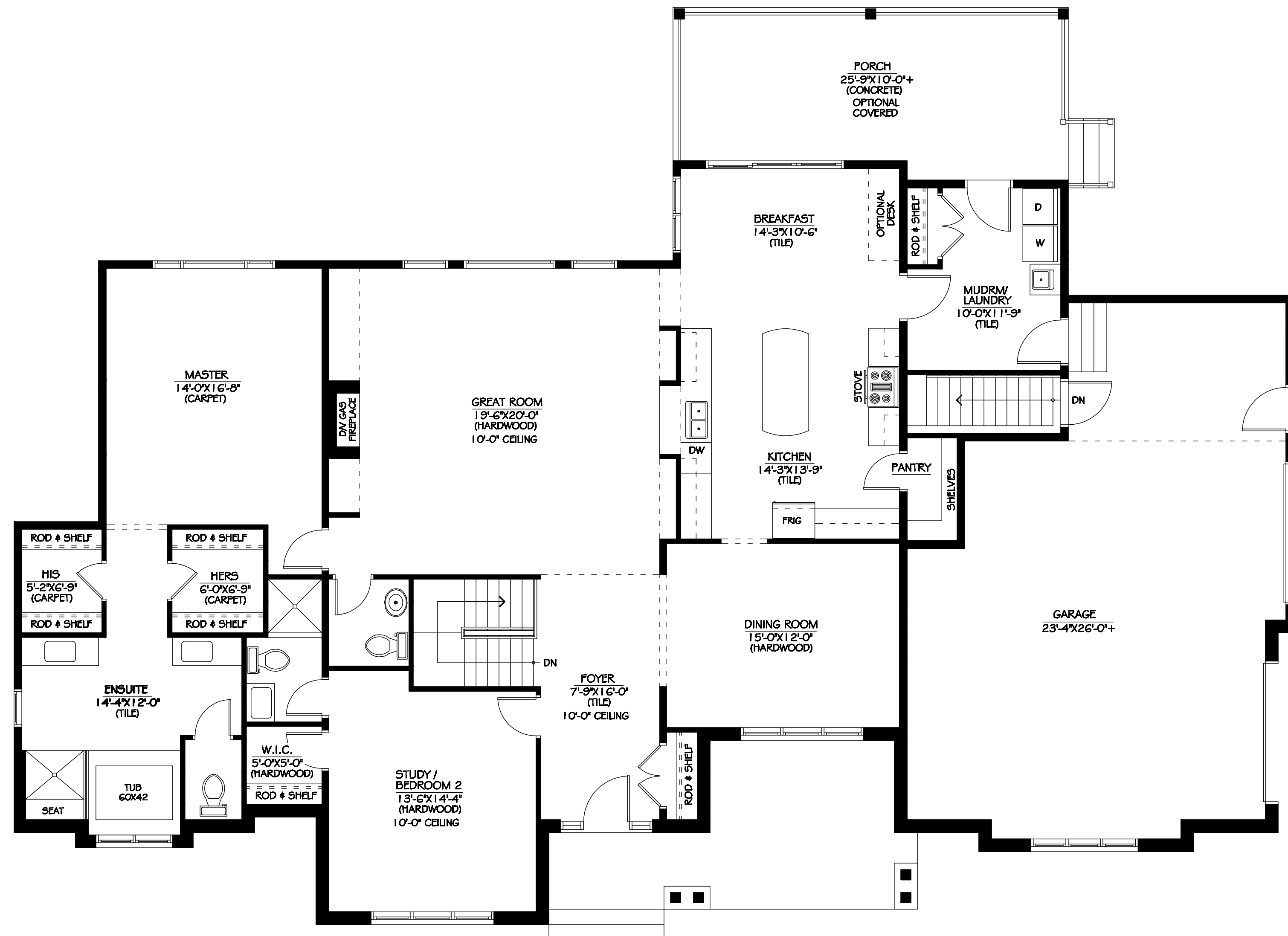
GROUND FLOOR 2395 SQ. FT.
